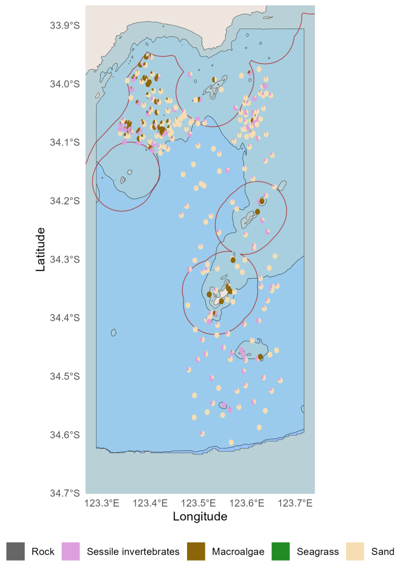
Figure 1: Habitat classes observed in spatially balanced stereo-BRUV and drop-camera (BOSS) imagery visualised as spatial pie charts, pooled across the 2022 and 2025 surveys. Commonwealth marine park boundaries are shown. The red line delimits state and commonwealth waters. Bathymetric contour at 30 m is shown.
