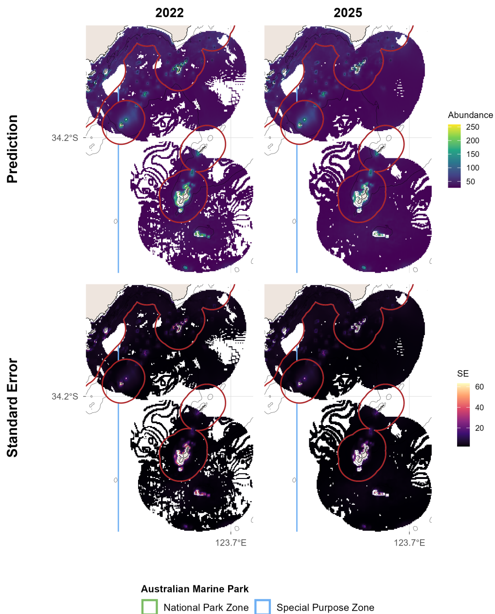
Figure 10.3: Demersal fish - Total abundance: spatial plots of distribution probability and uncertainty from stereo-BRUV groundtruthing. Commonwealth marine park boundaries are shown. The red line delimits state and commonwealth waters. Bathymetric contour at 30 m is shown.
