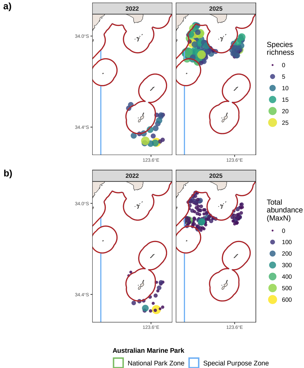
Figure 8: Spatial distribution of observed species richness and total abundance (MaxN) per stereo-BRUV deployment. Commonwealth marine park boundaries are shown. The red line delimits state and commonwealth waters.
