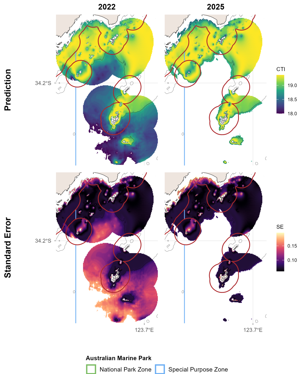
Figure 12.3: Demersal fish - Reef Fish Thermal Index: spatial plots of distribution probability and uncertainty from stereo-BRUV groundtruthing. Commonwealth marine park boundaries are shown. The red line delimits state and commonwealth waters. Bathymetric contour at 30 m is shown.
