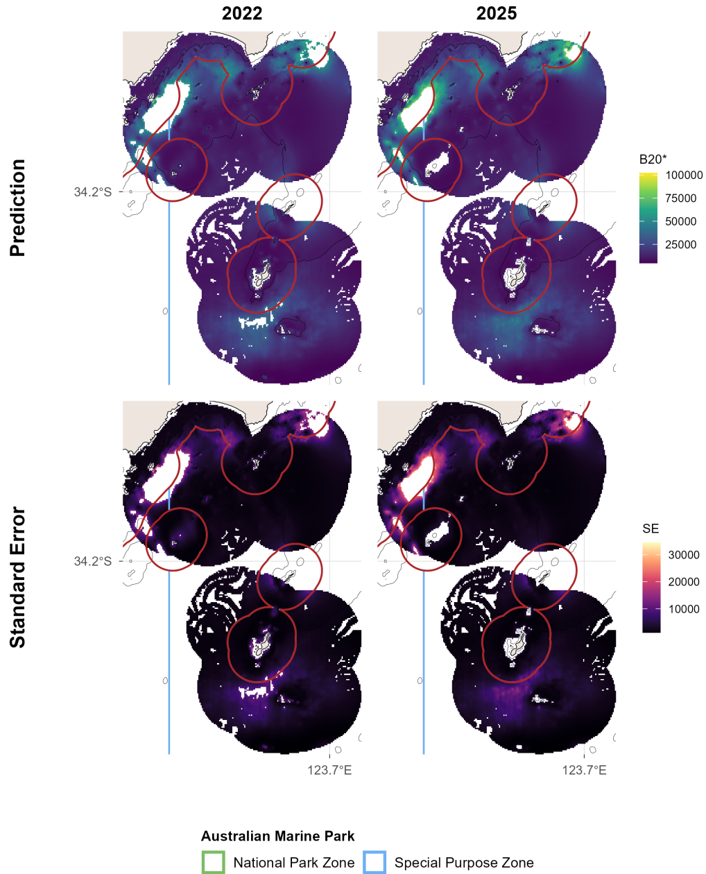
Figure 11.3: Demersal fish - Large Reef Fish Index*: spatial plots of distribution probability and uncertainty from stereo-BRUV groundtruthing. Commonwealth marine park boundaries are shown. The red line delimits state and commonwealth waters. Bathymetric contour at 30 m is shown.
